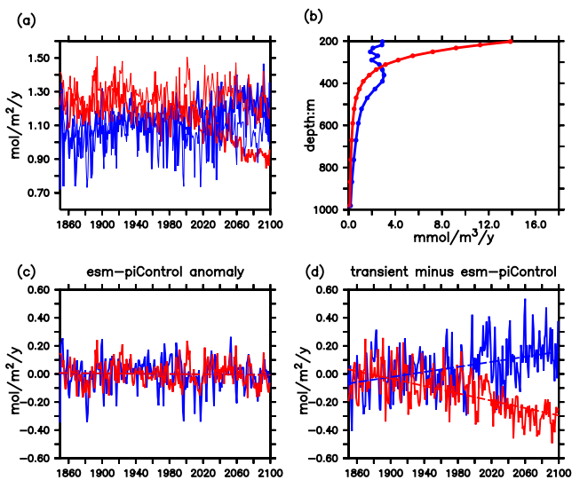
Figure 3. As Figure 2, but for the TSA section (see blue line in Figure 1d). In panel (b), all r^2 values of the linear regressions of apparent oxygen utilization against ideal age on density surfaces are above 0.94. The standard deviation of true respiration rates and oxygen utilization rate is too small to be visible.
