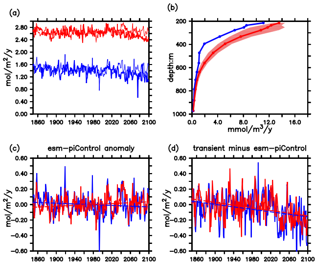
Figure 2. Comparison between vertically integrated oxygen utilization rate (OUR) and true respiration (200–1,000 m) along the NASG section (see blue line in Figure 1a) in simulation ensemble member 1. Panel (a) shows absolute vertically integrated OUR (blue) and true respiration (red) from the transient simulation (thick) and the esm-piControl simulation (thin). Panel (b) is the vertical distribution of OUR (blue) and true respiration (red) in the last year of the esm-piControl simulation. The shading indicates one standard deviation, while OUR standard deviation is too small to be visible. All r^2 values of the linear regressions of apparent oxygen utilization against ideal age on density surfaces are above 0.92. Panel (c) shows the integrated OUR (thick blue line) and true respiration (thick red line) anomalies relative to the respective time-averaged values of the esm-piControl simulation. The thin solid lines are the linear least square regression lines of integrated OUR anomalies (blue) and integrated true respiration anomalies (red) over time. Panel (d) shows the transient minus esm-piControl integrated OUR (blue) and true respiration (red), and their linear least square regression lines over time.
